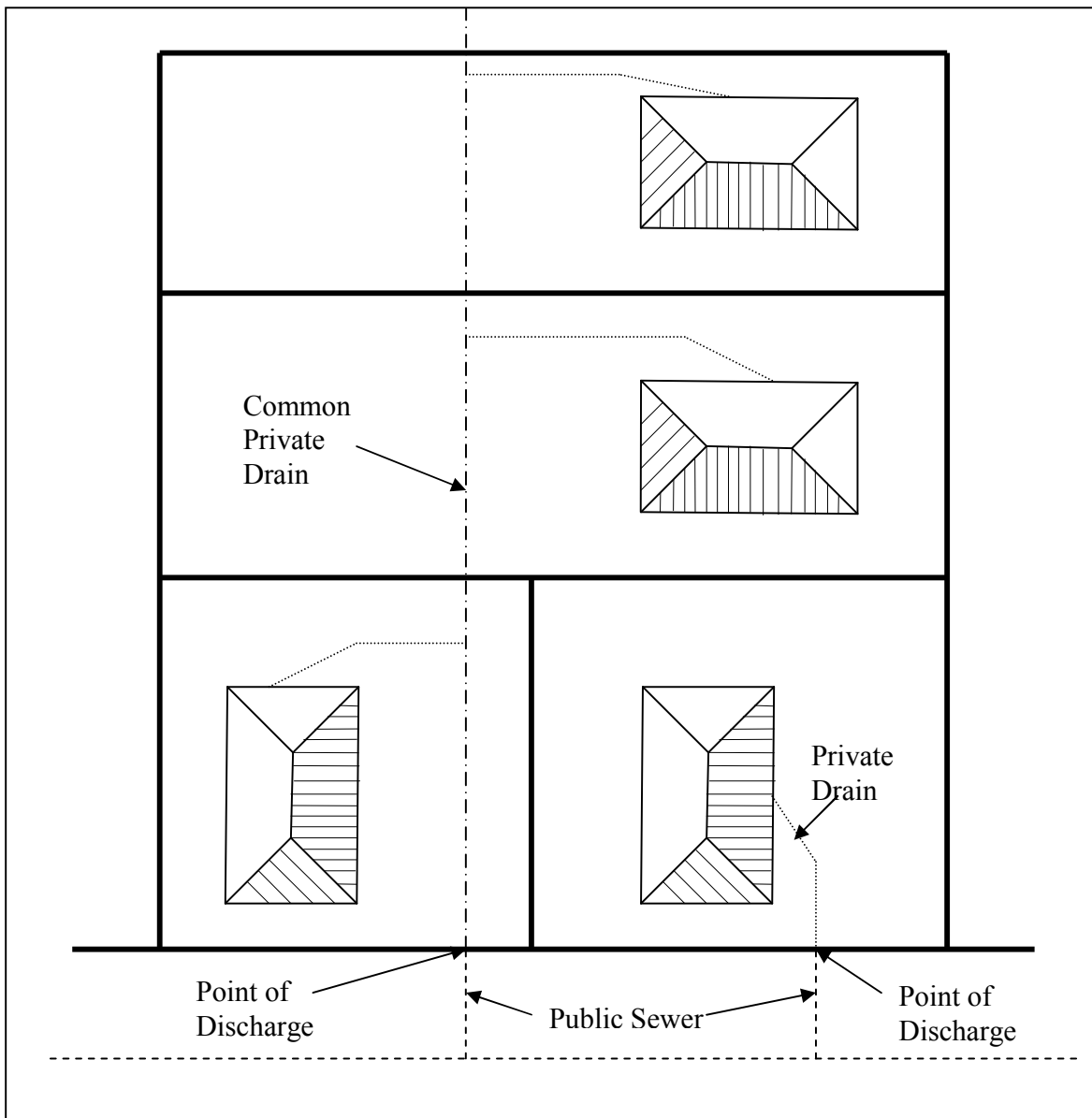
Figure 4 - Point of Discharge Location - Common Private Drain
