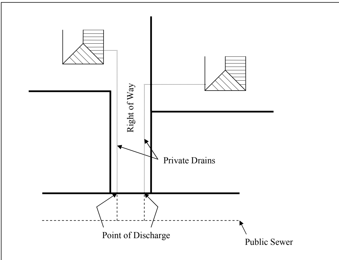
FIGURE 2 - POINT OF DISCHARGE LOCATION - REAR LOTS
