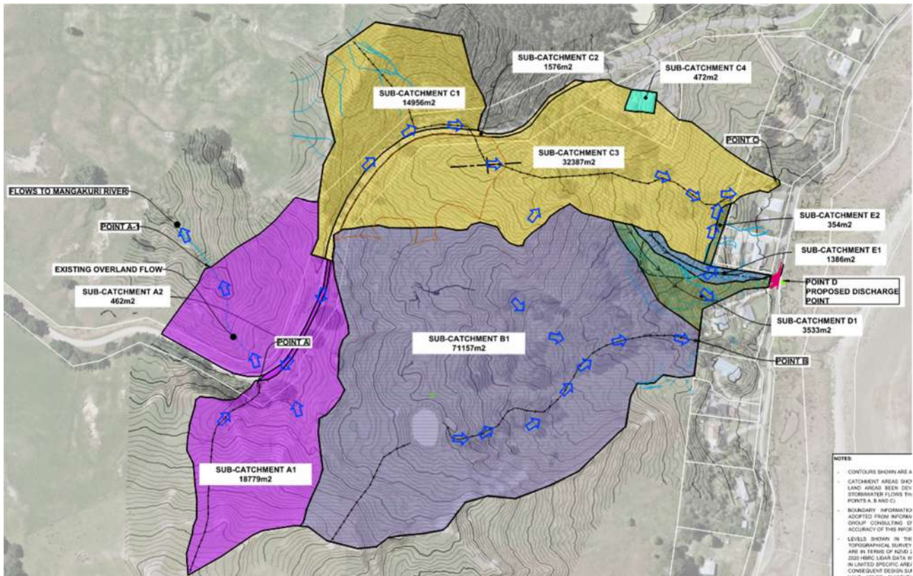
Figure 9 - Pre-development stormwater Catchments and main discharge points
